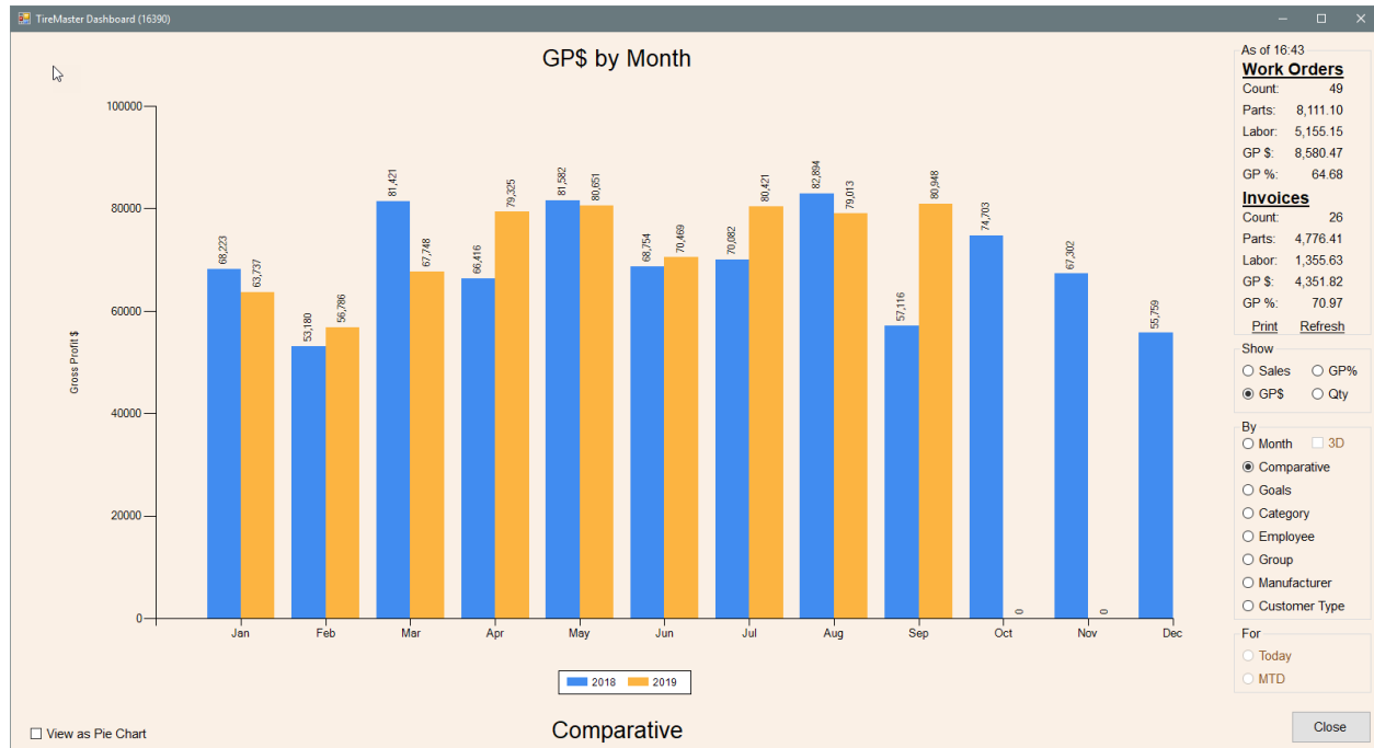
Figure 33-1: TireMaster Dashboard
